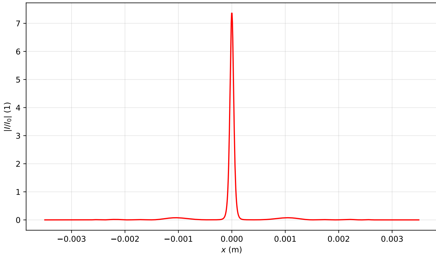
Intensity profile I(x, y = 0, z = 0.796)/I_0 , P_{in}=7.0P_{cr} , artificial time
